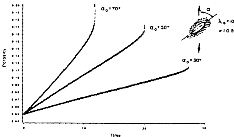
Fig. 7. Evolution of porosity of various initial voids positions. Different growth rates are exhibited ( \lambda_0 = 10, n = 0.5, f_0 = 5\% ).
